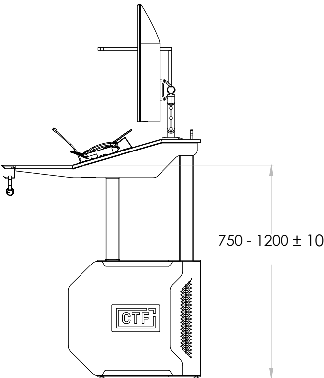
SIDE VIEW
